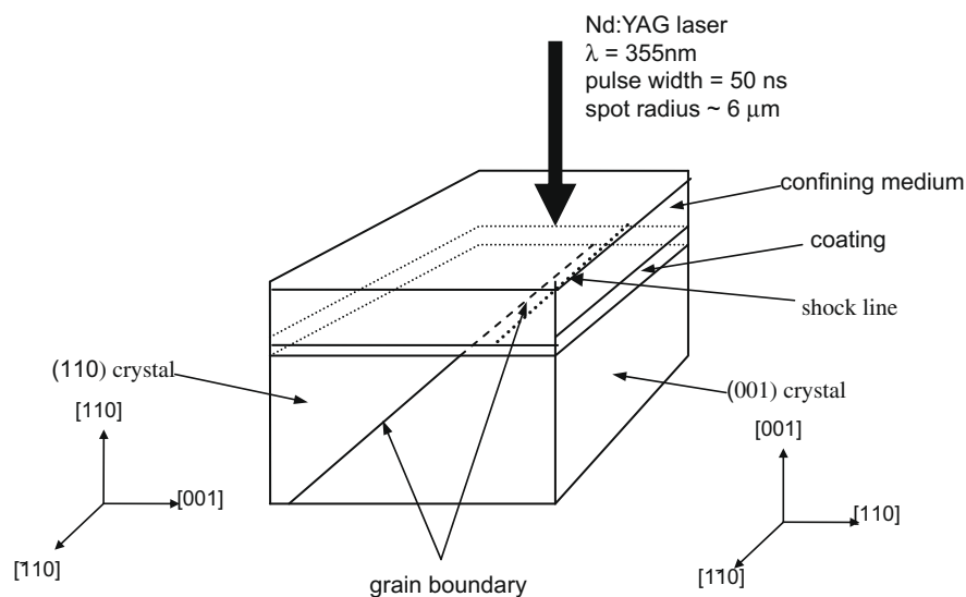
Fig. 2. Experimental setup.
