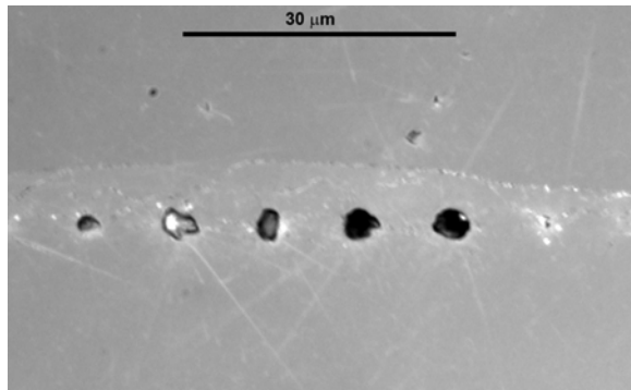
Figure 2. Refractive DIC optical microscopy of top view (xy-plane) of the new polished surface across the channels irradiated by a series of single pulse energy of 30 \mu\text{J} .
