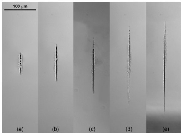
Figure 5. Transmission DIC optical microscopy of cross section view (xz-planes) of features and channels using same pulse energy of 30 \mu\text{J} at different focusing depths of (a) 500 \mu\text{m} , (b) 1000 \mu\text{m} , (c) 1500 \mu\text{m} , (d) 2000 \mu\text{m} , and (e) 3000 \mu\text{m} . The above five figures have been adjusted to the same scale.
