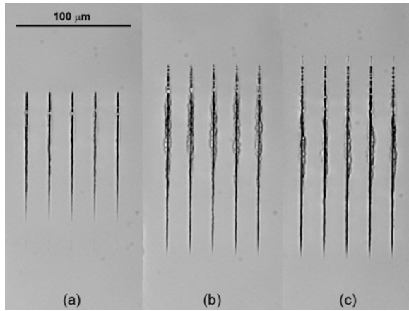
Figure 1. Transmission DIC optical microscopy of cross section view (xz-planes) of features and channels at same focusing depth of 1500 \mu\text{m} using pulse energy of (a) 10 \mu\text{J} , (b) 20 \mu\text{J} , and (c) 30 \mu\text{J} . The above three figures have been adjusted to the same scale.
