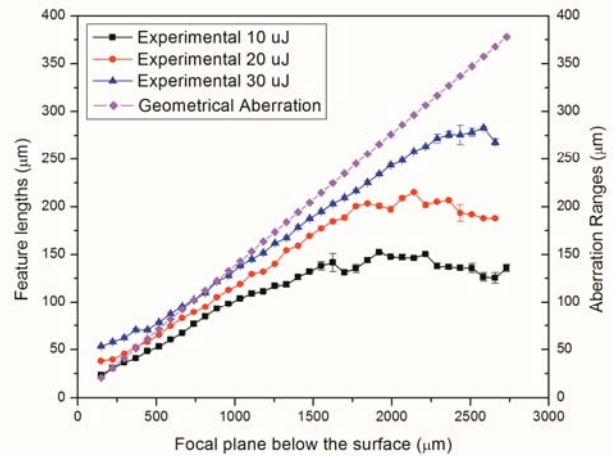
Figure 6. Comparison of experimental feature lengths at 10 \mu\text{J} , 20 \mu\text{J} , and 30 \mu\text{J} , and the paraxial aberration range at different focusing depths. Error bars denote standard deviation.
