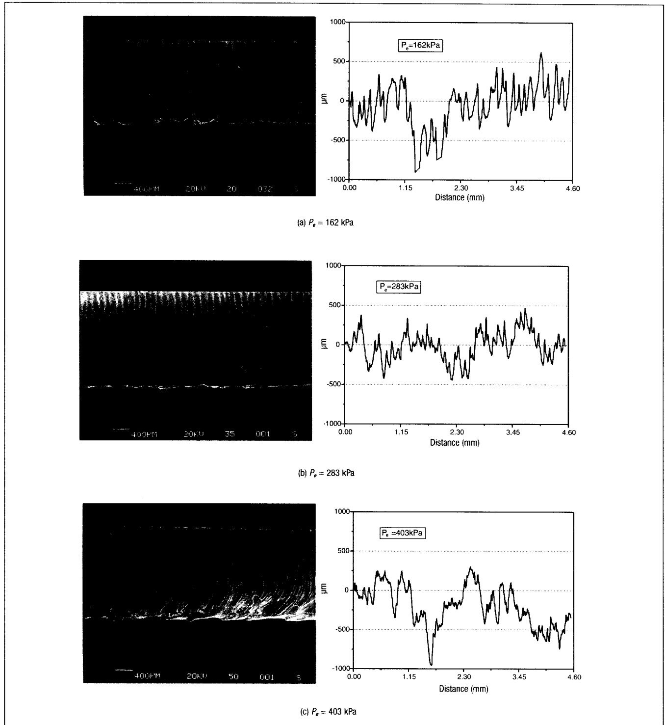
Figure 15 SEM and Profilometer Measurements of Cut Surface with Different Gas Pressure at 2.0 mm Standoff (laser power: 200 W; cutting speed: 40 mm/s; material thickness: 1.6 mm; oxygen assisted; incomplete cuts at P_g = 323 kPa, P_g = 363 kPa)
