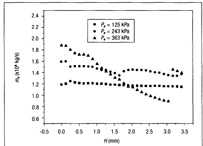
Figure 11 Variation of Through-Slot Mass Flow Rate Measurements with Standoff Distance for L = 1.1 mm
